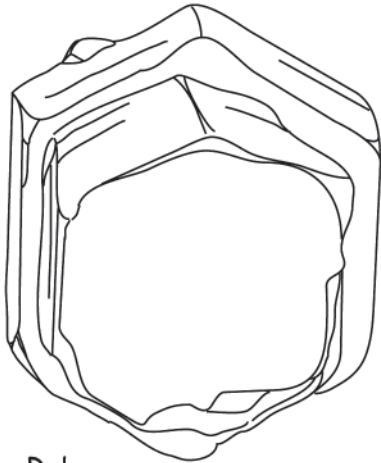
Ruby (Color: red)
